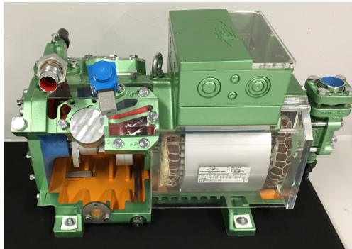
4NC-20.2Y (cutaway model)
