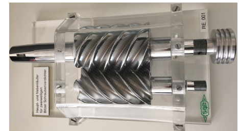
Male rotor and female rotor
